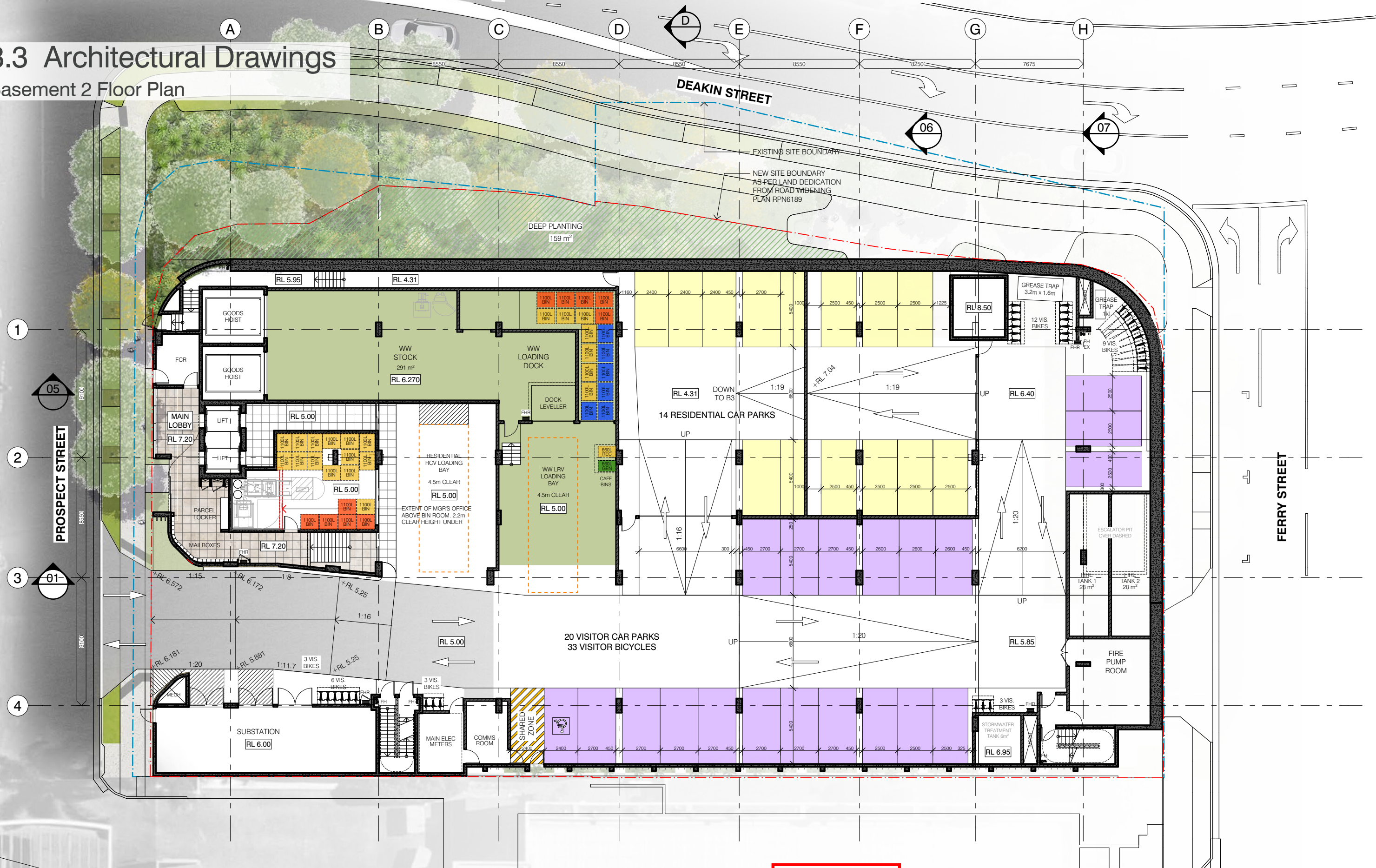
BASEMENT 2 FLOOR PLAN - 1:250 (A3)
