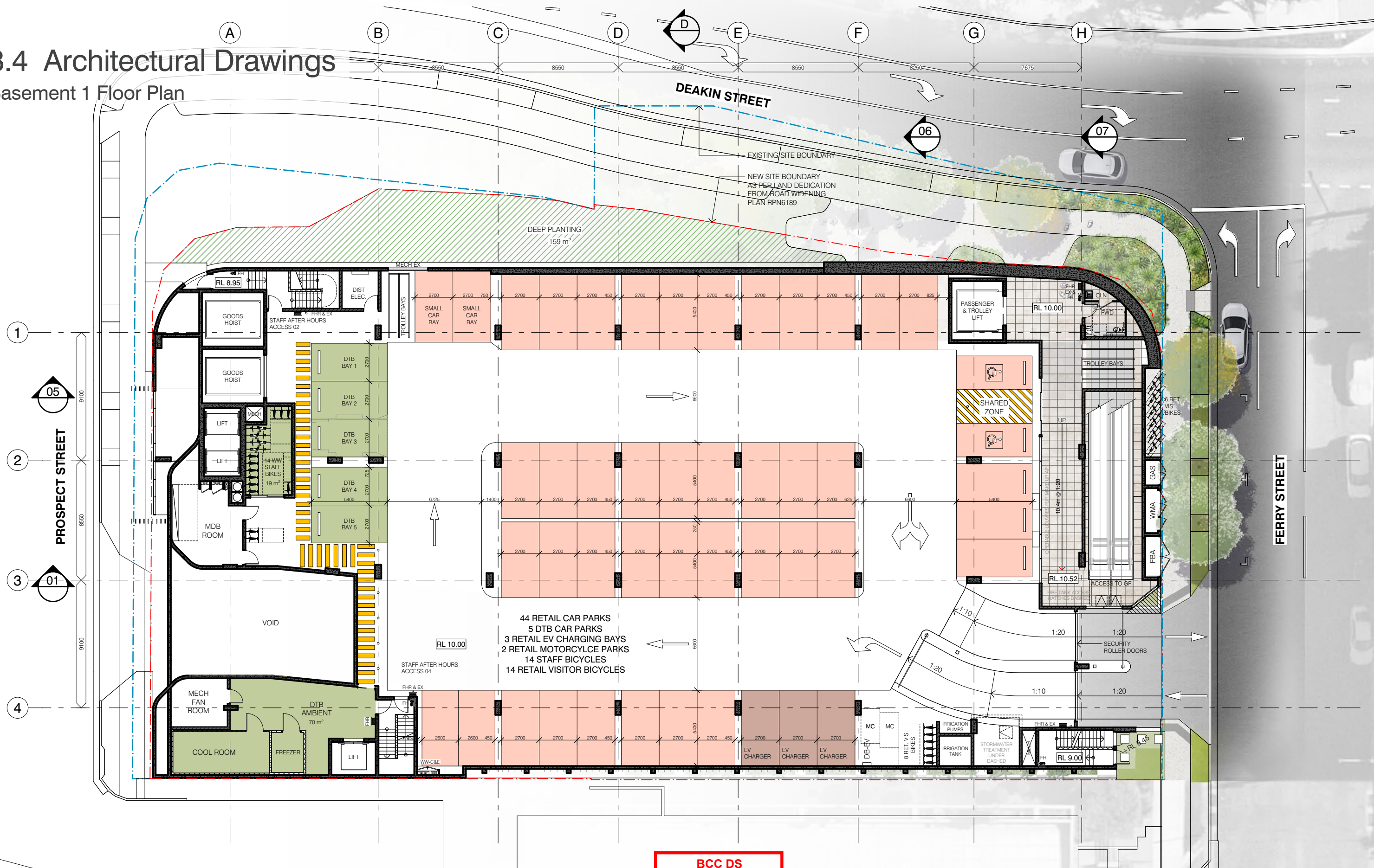
BASEMENT 1 FLOOR PLAN - 1:250 (A3)
