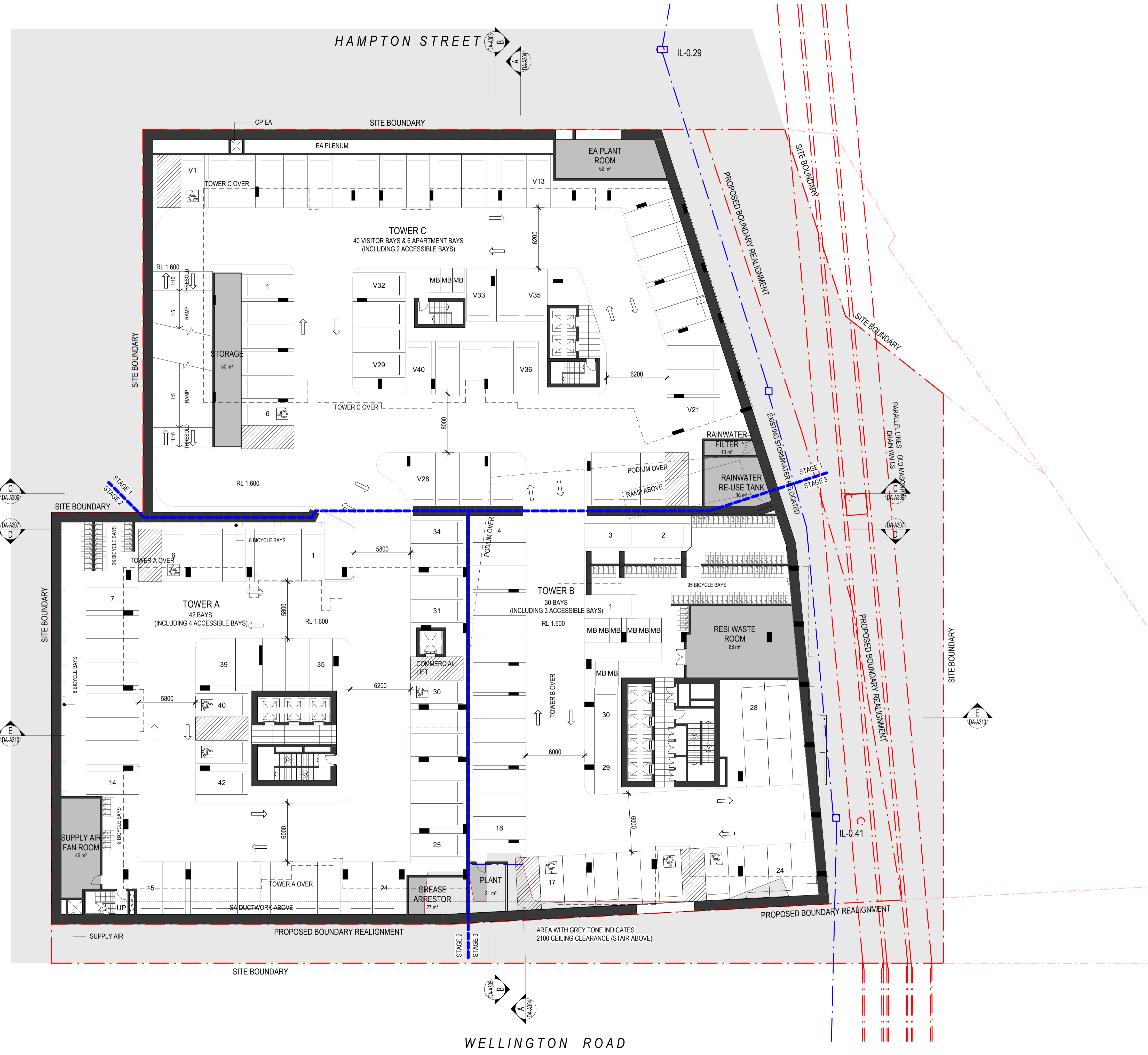
1 BASEMENT 1 1: 200 @ A1
