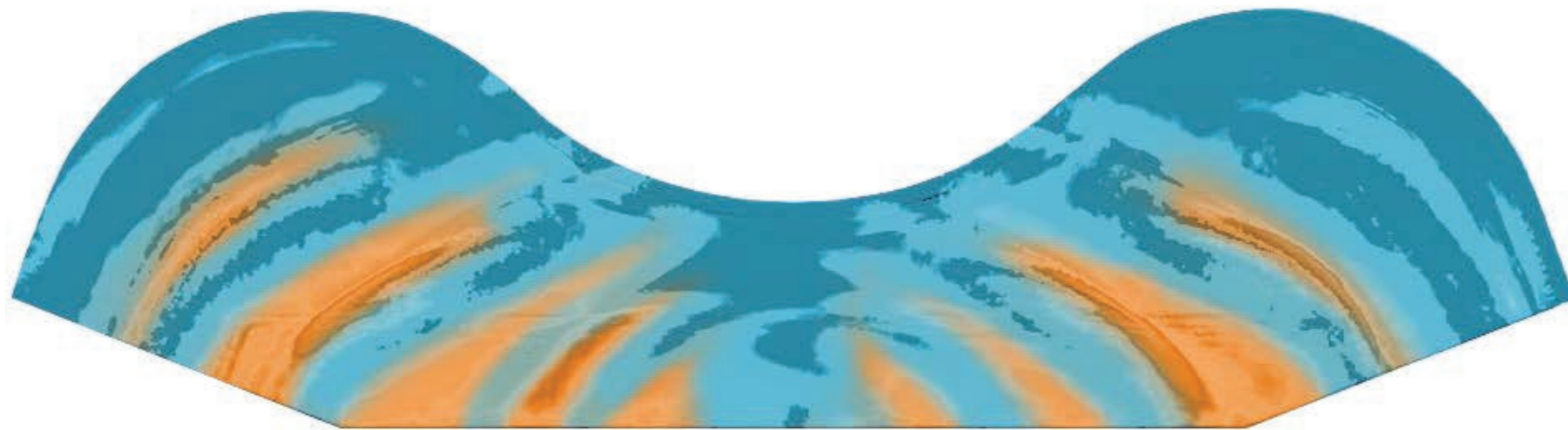
Endless Surf wave simulation
